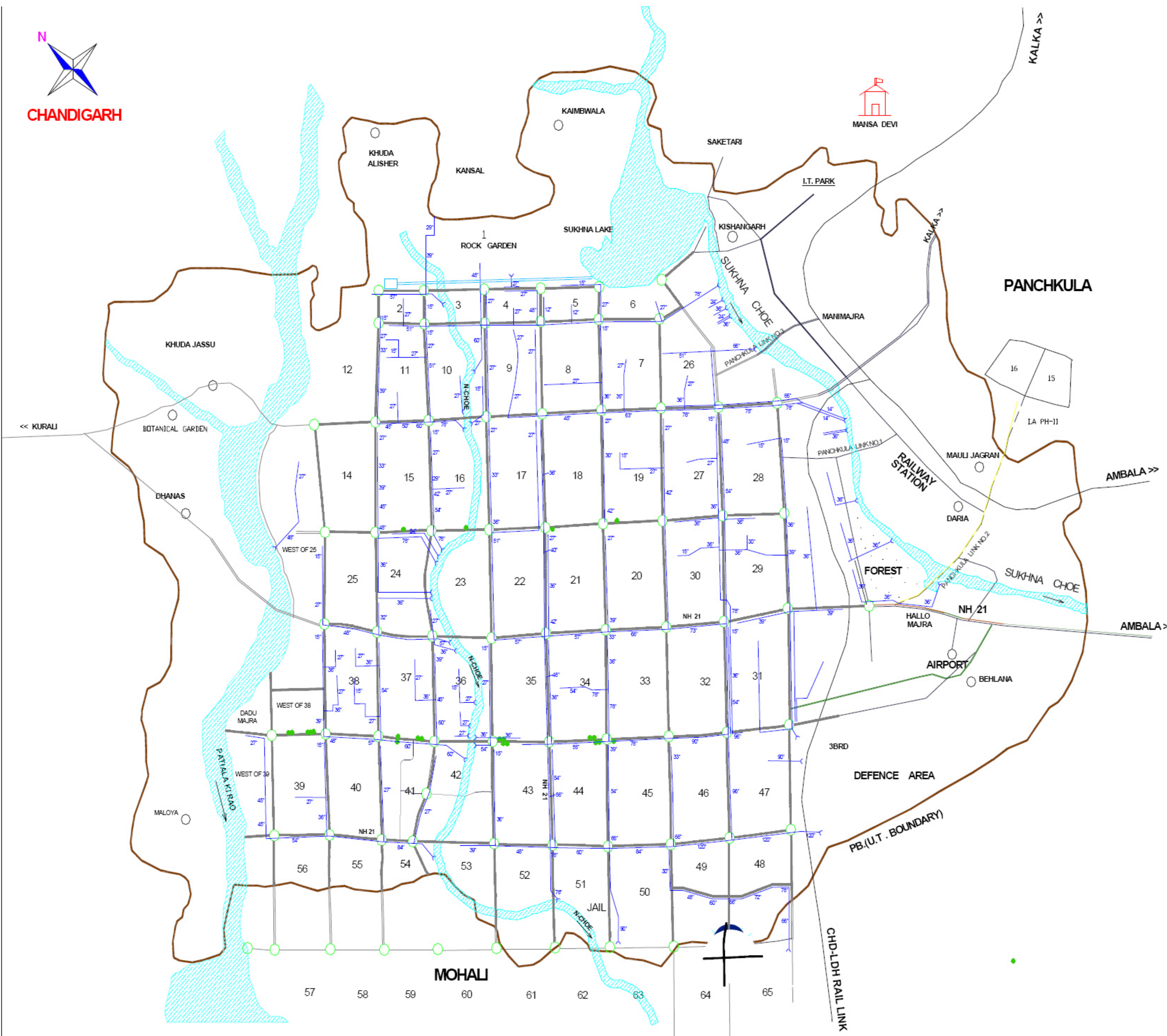
PLAN SHOWING OF STORM WATER DRAINAGE SYSTEM FOR CHANDIGARH TOWN
